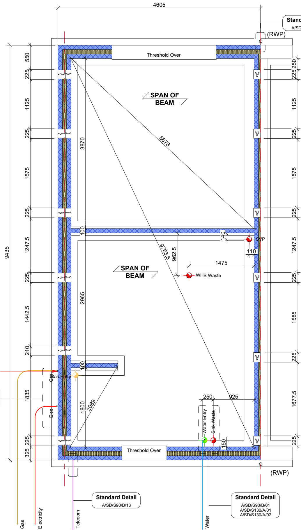
1 Foundation - Semi Detached 1 : 50
